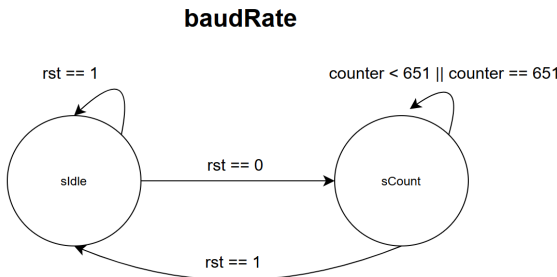
Figure 3.5: Write Baud Rate Generator FSM
