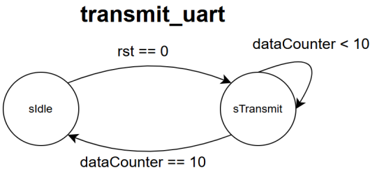
Figure 1.3.1: transmit_uart FSM
