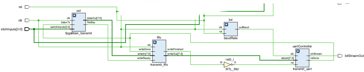
Figure 2.3: Complete UART Write Block Diagram
