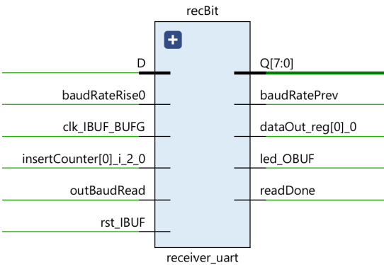
Figure 1.3.4: receiver_uart Block Diagram
